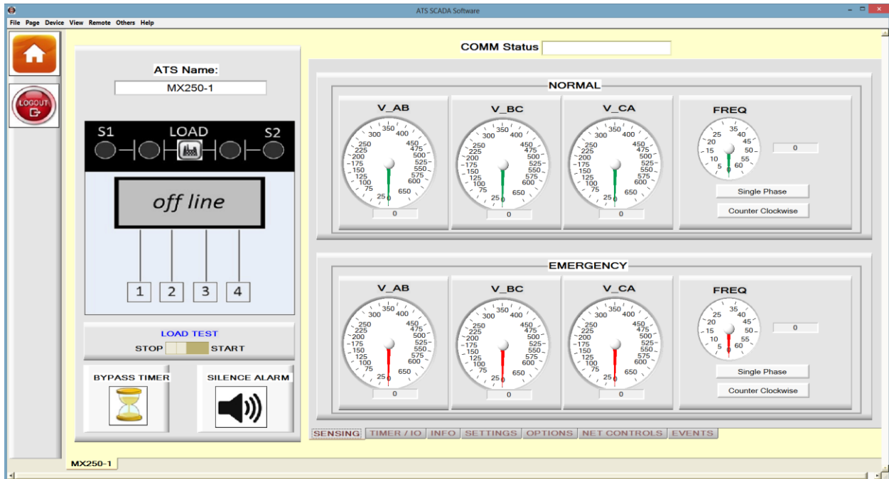
Fig 2 – MX250 (Sensing)
